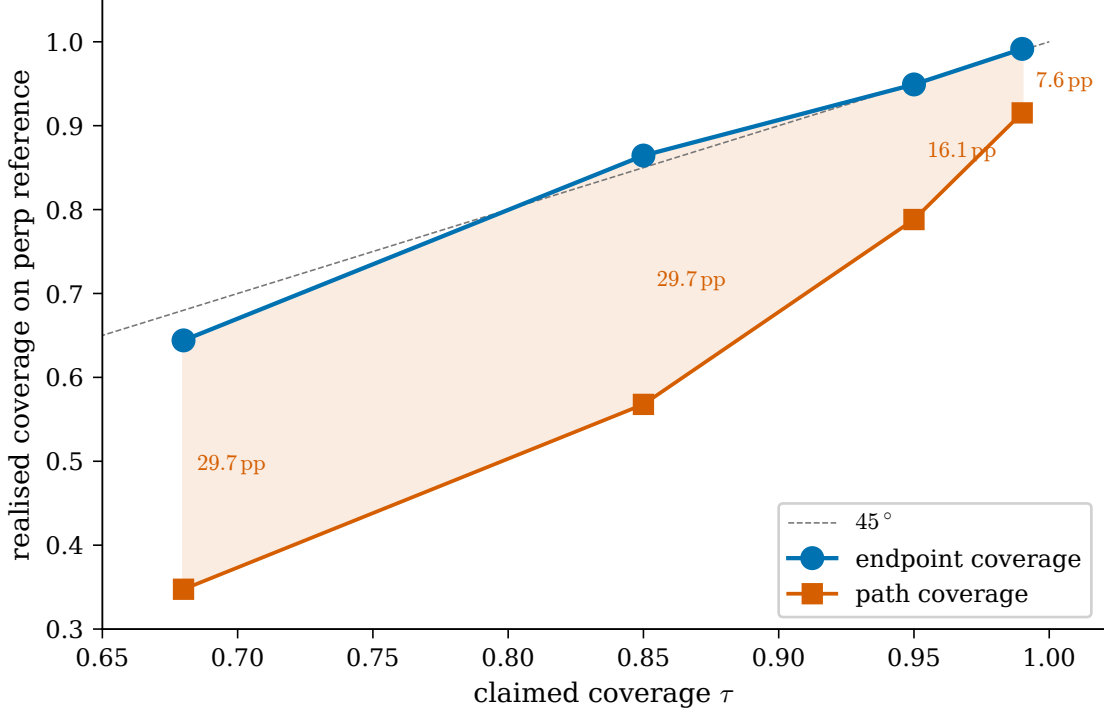
Figure 9: Path coverage gap on the 24/7 stock-perp reference. Endpoint coverage (blue) tracks nominal across \tau \in \{0.68, 0.85, 0.95, 0.99\} on the perp-listed subset; path coverage (vermillion) — the fraction of weekends where the perp 1m bar high/low stay inside the served band over the full [Fri 16:00, Mon 09:30] window — runs 29.7/29.7/16.1/7.6 pp behind. The gap collapses meaningfully only at \tau = 0.99 . Sample is small ( n = 118 symbol-weekends across 19 calendar weekends, 2025-12 to 2026-04); the read is directional and §10.2 (the path-fitted conformity score) is the methodology fix.
